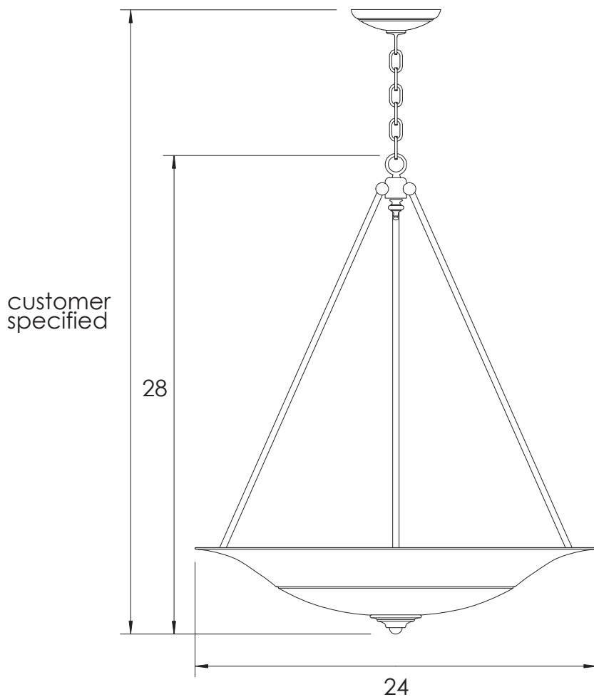
F1890 Uplight Chandelier three 100-watt halogen lamps
